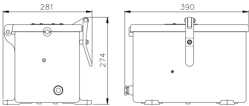
A4025 Stowage Box Weight 9.9Kg NSN6240-99-932-6625
